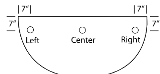
Half-Round 48" or 60"
