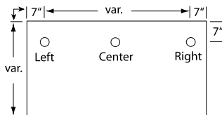
Rectangular 24" or 30"
